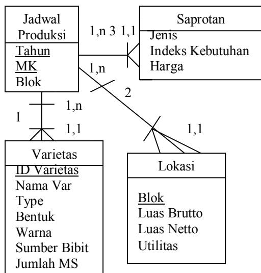
Gambar 2. Diagram Entity Relationship SIMPro
